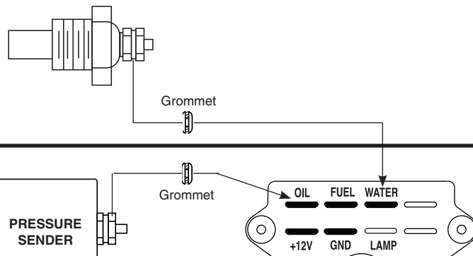
TEMPERATURE SENDER
