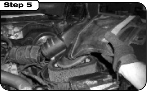
Remove top half of air box from lower half. Remove factory intake tube from factory turbo inlet elbow.
