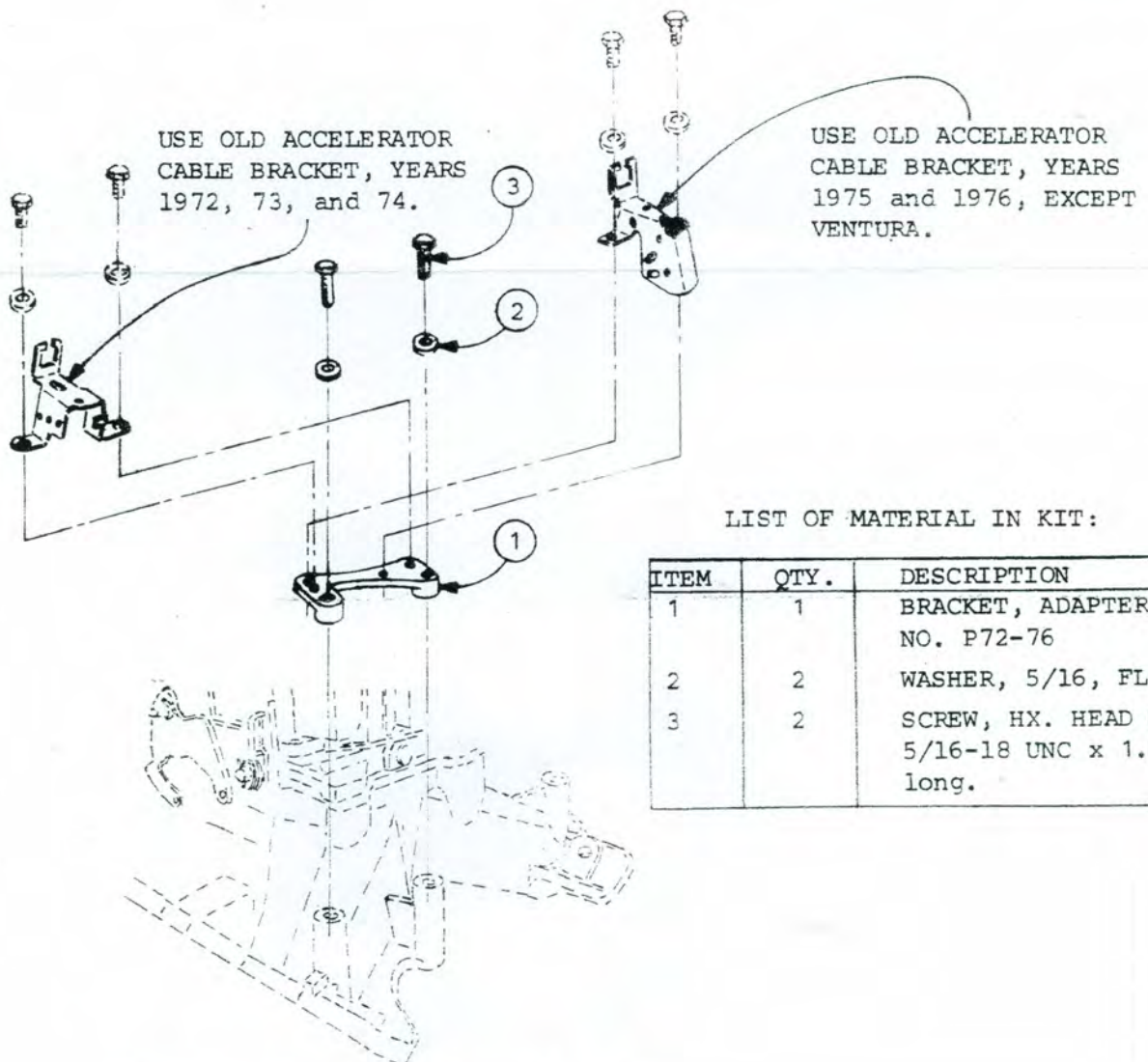
FIGURE 1, ASSEMBLY OF PARTS FOR ALL PONTIACS 1972 THRU 1976.
