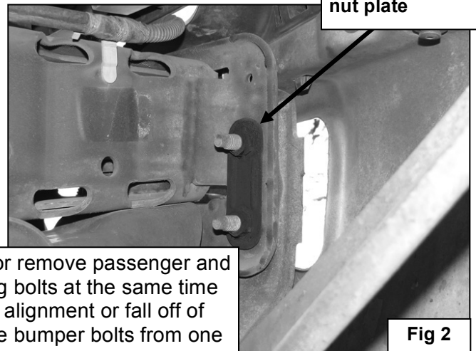
Factory double nut plate
