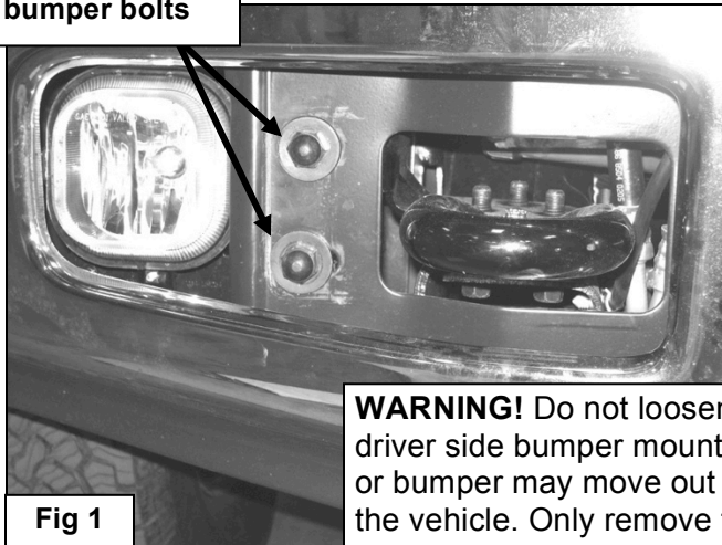
Remove factory bumper bolts
