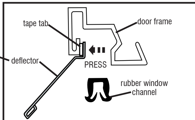
Cross Section Of Deflector In Place
